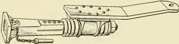
Fig. 119. Drawbar of a Simple Coupler
